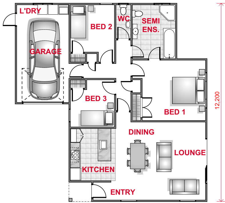
FLOOR PLAN
