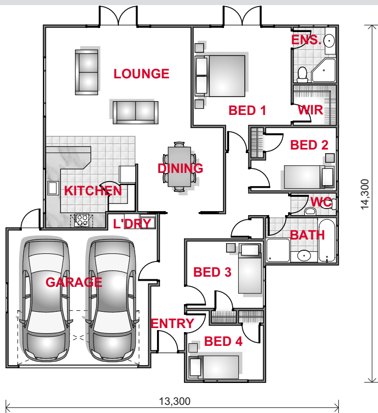
FLOOR PLAN
